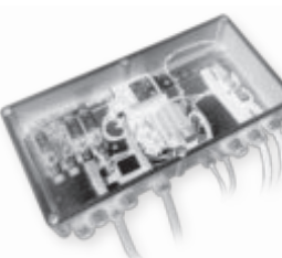
The DC Distribution cabinet controls the Lithium Ion batteries. It contains the DC fuses, shunts, 300A safety relay, and controls the cell-balancing, charging and discharging of the system. The DC Distribution cabinet is pre-wired for your application, it saves your installation time and protects the battery pack against overcharging and discharge.
